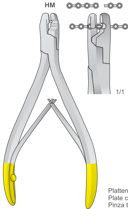
Plattenschneidezange Plate cutting Pliers Pinza taglia placche
