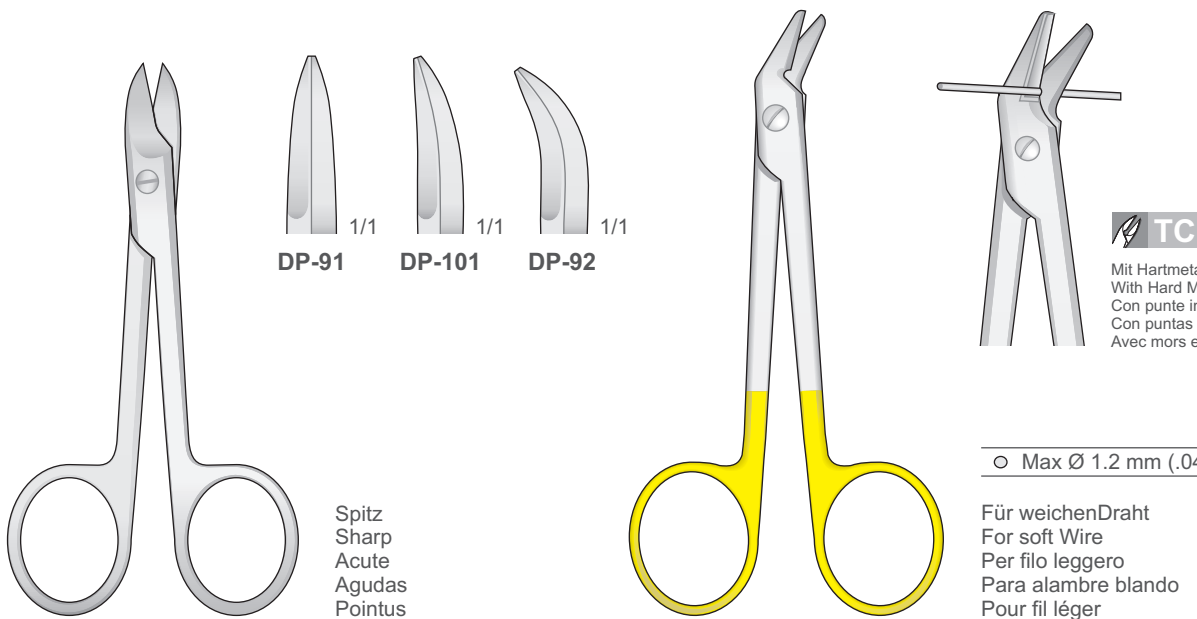
BEEBE DP-91/DP-101 110 mm
